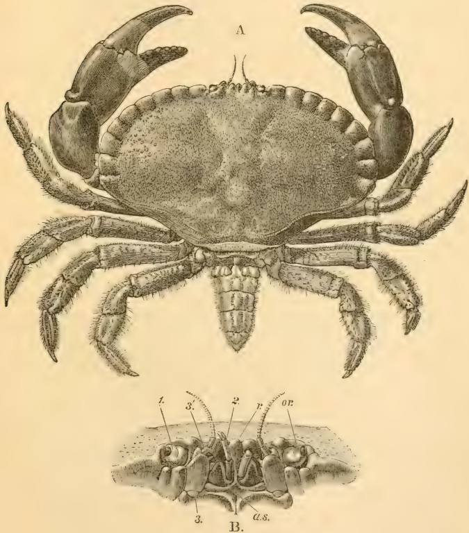
FIG. 72. Cancer pagurus , male ( \frac{1}{3} nat. size). A, dorsal view, with the abdomen extended; B, front view of "face." a.s. , antennary sternum; or. , orbit; r. , rostrum; 1. eyestalk; 2. antennule; 3. base of antenna; 3', free portion of antenna.
